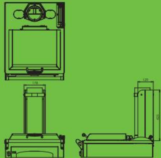
BakeChef Cooking Stove Flue Heatshield Assembly
