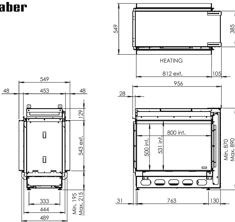
Dimensional Drawing e-Matrix Mood 800/500 ST
